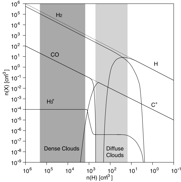
Fig. 6. Schematic of the number density variation of H_3^+ with respect to hydrogen along with that of major molecules and ions in the interstellar medium. The number density of H_3^+ is independent of n(H) , in contrast with the other molecules. We define “dense” and “diffuse” clouds by the form of carbon atoms. The form of carbon is critical, since it defines the destruction mechanism of H_3^+ , and hence the number density of the molecular ions.
