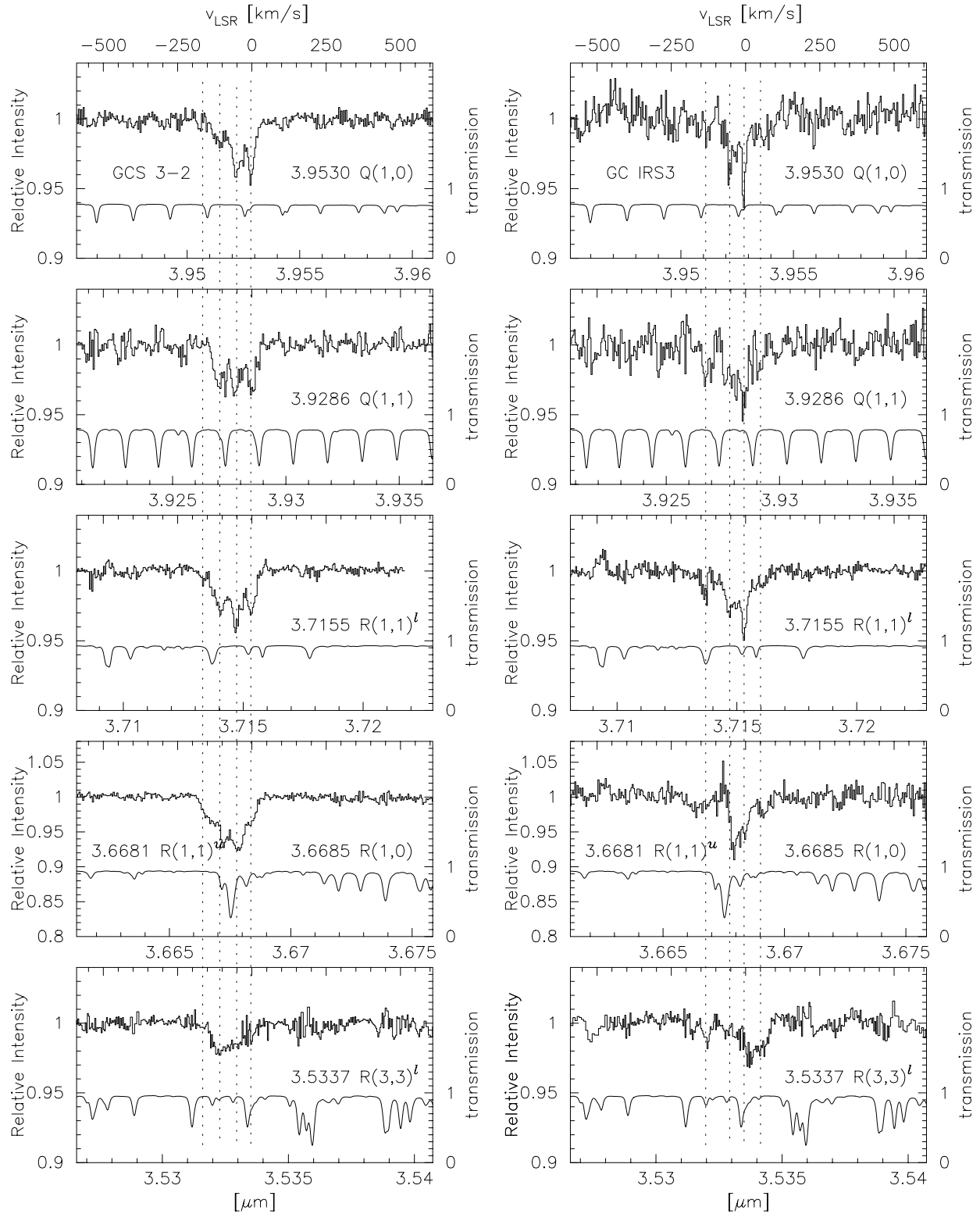
Fig. 2. Total detected H_3^+ absorption spectra toward GCS 3-2 (left column) and GC IRS 3 (right column). Kinematic components are indicated in the LSR velocity by dotted lines (see figure 4). Note that the 3.668 \mu\text{m} line profile appears to be different from the others because it consists of a close doublet of R(1, 0) and R(1, 1)^u separated by \Delta v = 35 \text{ km s}^{-1} . The feature is lined up with other absorption lines at R(1, 0) 3.6685 \mu\text{m} . The model atmospheric transmission curves are shown to discriminate the genuine detections from the possible artifacts of the poor cancellation of the telluric absorption lines.
