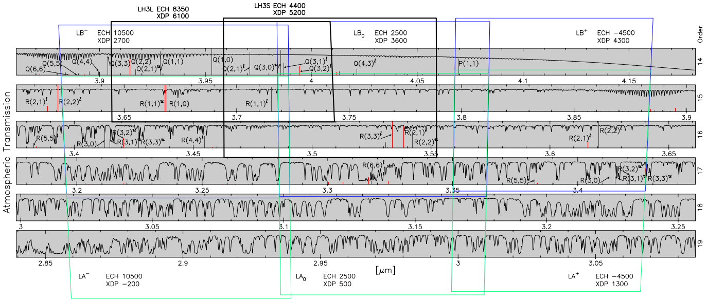
Fig. 1. Wavelength coverage of the IRCS echelle mode in the 3\ \mu\text{m} region. The entire L -band ( 2.84\text{--}4.18\ \mu\text{m} ) is covered by six standard settings ( \text{LA}^- , \text{LA}_0 , \text{LA}^+ , \text{LB}^- , \text{LB}_0 , \text{LB}^+ ; shown in green and blue rectangles), but 70% is covered by three settings. “ECH” and “XDP” denote the angles of the echelle and the cross-disperser gratings. The grating angle can be seamlessly modified so as to be best suited to individual projects. The two settings which we employed for the observation are shown by the bold-line enclosures. The positions of the major \text{H}_3^+ lines are indicated by sticks with the heights representing the relative intensities calculated with T = 300\ \text{K} . The atmospheric transmission curve is overlaid to illustrate the region where the interference of the telluric atmospheric absorption is severe.
