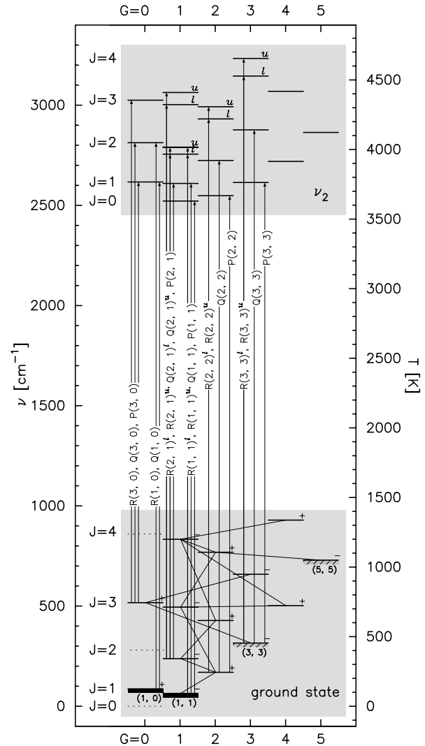
Fig. 7. Rotational energy levels of H_3^+ in the ground state and in the \nu_2 vibrationally-excited state. H_3^+ has two vibrational modes of which only \nu_2 is infrared-active, and targeted in our observation. G = |k - l_2| is used instead of K in the diagram, where l_2 is a vibrational angular momentum of \nu_2 . G is a better quantum number than K where l_2 \neq 0 (see McCall 2001 for details). The letters u and l marked in the \nu_2 state denote the levels of the same G number, but with different combinations of k and l_2 . The major transitions of \nu_2 \leftarrow 0 that appear in the 3 to 4 \mu\text{m} regions are indicated by the vertical connecting arrows with labels. Note that for the ground vibrational state, the J = 2n and G = 0 levels are forbidden by the Pauli principle (shown in dotted bars). The lowest levels of ortho- (J, G) = (1, 0) and para- (J, G) = (1, 1) H_3^+ are marked with thick solid bars. The selection rules allow only radiative relaxation between two levels that satisfy \Delta J = 0, \pm 1 and \Delta G = \pm 3 . The spontaneous transitions are indicated with connecting lines of energy levels in the ground state. The transition between G = 2 \leftrightarrow 1 can be understood to be G = \pm 2 \leftrightarrow \mp 1 . The “+” and “-” signs in the ground state denote the parity of the energy levels. The parity rule, + \leftrightarrow - , is automatically satisfied by \Delta G = \pm 3 . The (J, G) = (3, 3) and (5, 5) are disconnected from any lower levels by the selection rule, making the two levels metastable (Pan, Oka 1986). The (4, 4) level can relax to (3, 1) , but has a long lifetime.
