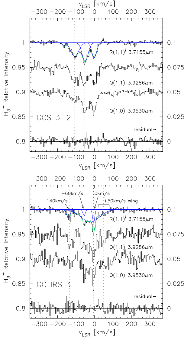
Fig. 4. Gaussian decomposition of the kinematic components for GCS 3-2 (top) and GC IRS 3 (bottom). At least four components are found in ortho- Q(1, 0) and para- R(1, 1)^l and Q(1, 1) \text{H}_3^+ absorption lines at common velocities. The residual of the fitting is shown at the bottom of each panel. The decomposition parameters are summarized in table 3.
