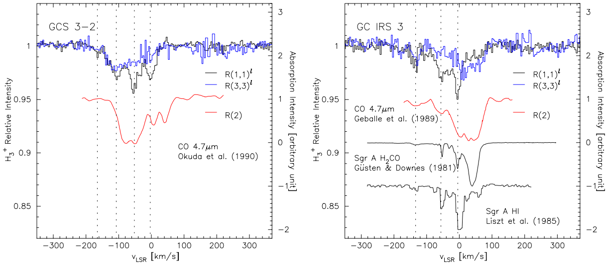
Fig. 5. Comparison of the line profiles of \text{H}_3^+ at R(1, 1)^l and R(3, 3)^l along with those of other species toward the same objects. GCS 3-2 is on the left, and GC IRS 3 on the right. The absorption spectra from previous studies are shown in arbitrary units. The dotted lines represent the velocity components of the R(1, 1)^l transition in the previous figure. Three velocity components in GC IRS 3 at -140 \text{ km s}^{-1} , -60 \text{ km s}^{-1} , and 0 \text{ km s}^{-1} match well with CO R(2) , \text{H}_2\text{CO} , and \text{HI} absorption, indicating the same absorbing clouds. The deep absorptions of CO and \text{H}_2\text{CO} at +50 \text{ km s}^{-1} toward the Galactic center do not correspond to strong components in the \text{H}_3^+ spectrum, which might be accounted for by the compact structure of the absorbing cloud. Note the considerable difference in the line shape of R(3, 3)^l from R(1, 1)^l for both GCS 3-2 and GC IRS 3. The line profile of the R(3, 3)^l in GC IRS 3 is more or less similar to that of CO absorption at 4.7 \mu\text{m} .
