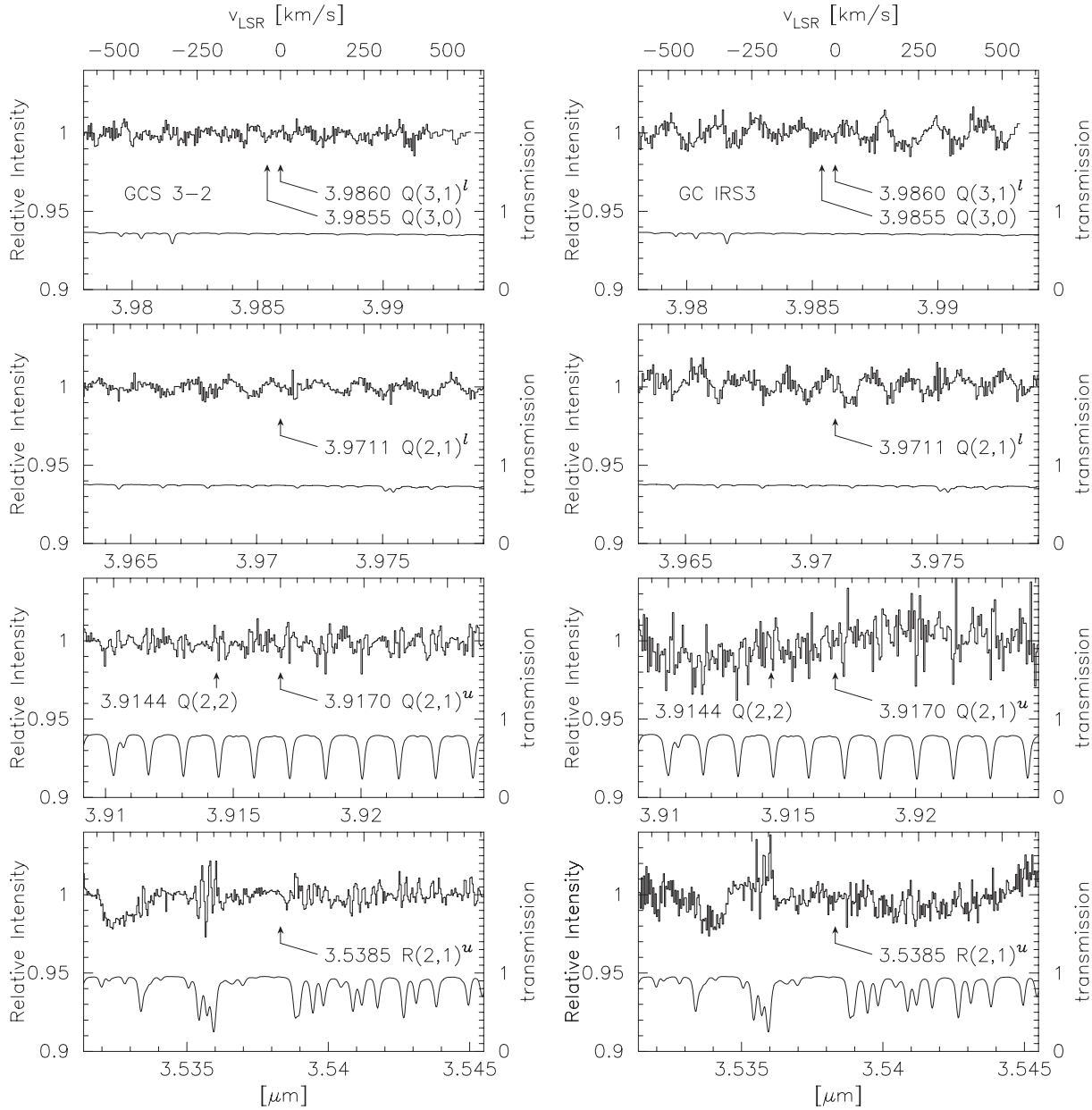
Fig. 3. Same with figure 2, but for negative detections. The periodic patterns seen at 3.97–3.99 \mu\text{m} are instrumental fringes left unprocessed. Note that the dips at 3.534 \mu\text{m} in the bottom panels are R(3,3)^l positively detected.
