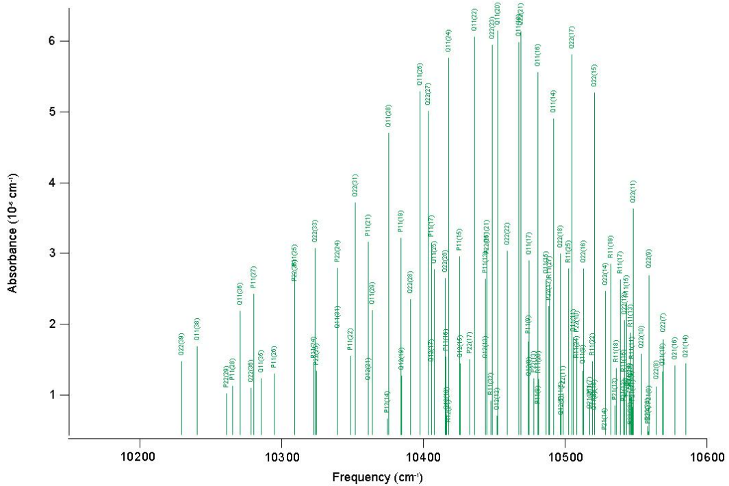
Figure 7: Assigned spectrum of N 2 +
