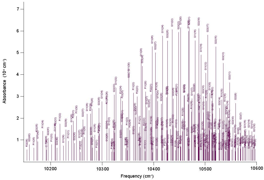
Figure 6: Predicted Spectrum of N 2 +
